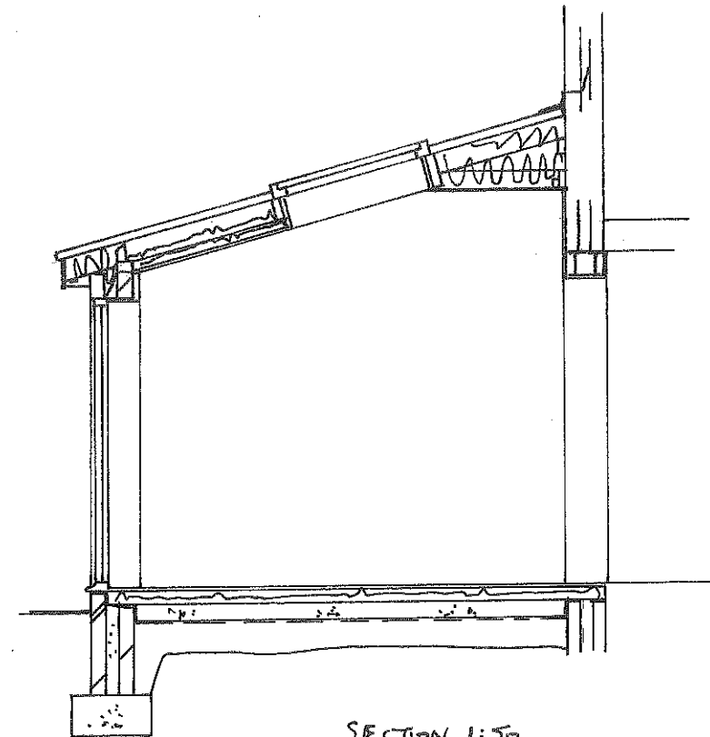
SECTION 1:50
